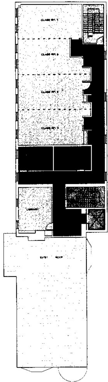
THIRD FLOOR PLAN SCALE 8" = 1'-0" GROSS AREA 3445 SQFT NET AREA 2769 SQFT
